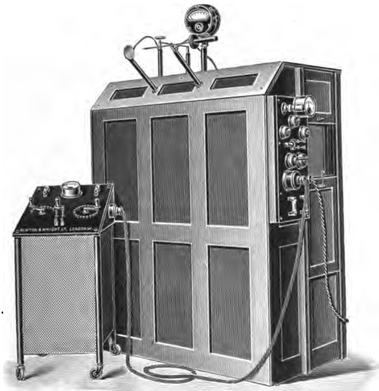
The "Snook" Röntgen apparatus.
